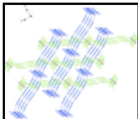
Fig. 3. The three-dimensional structure built from two-dimension mutual inclined interpenetration of the compound (I).
